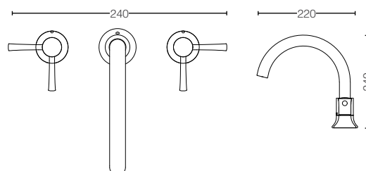
TBS02201B Bath Filler (3 Hole) Size : 240W x 220D x 249H mm
