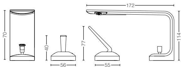
TLP02301B Single Lever Lavatory Faucet w/ Pop-Up Waste Size : 56W x 172D x 114H mm
